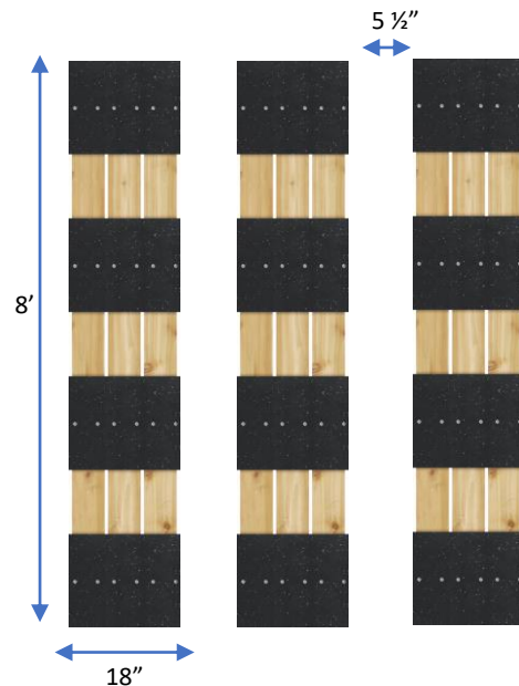
Fig 4. Arrange the panels 5 1/2" apart.
