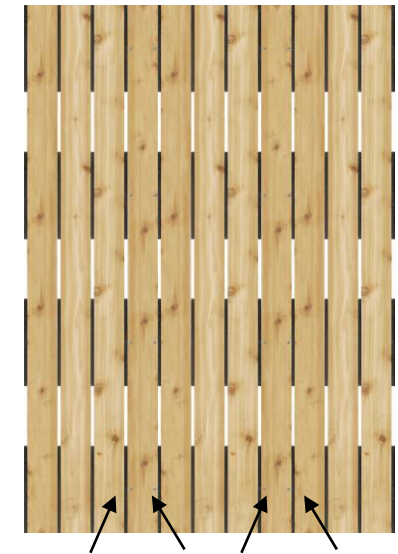
Fig 6. Screw joiner board to the rubber side supports.
