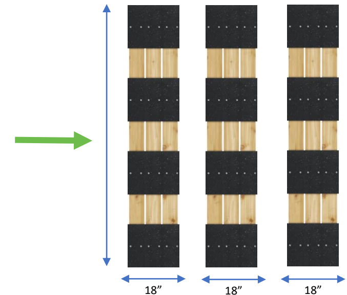
Fig 3. Build three identical panels.
