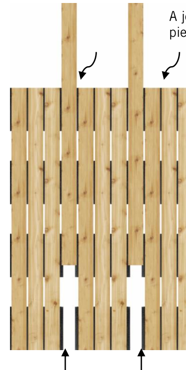
Fig 5. Insert joiner board into this 5 1/2" space indicated by the arrow.
