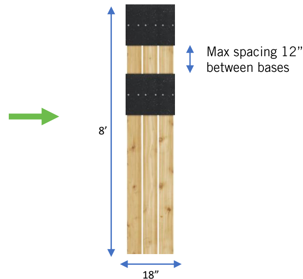
Fig 2. Space the bases max 12" apart.
